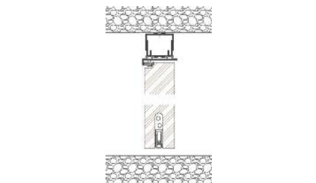
HT2 1000 Holztüre 2-flügelig D = 54 mm Rw = 34 dB
