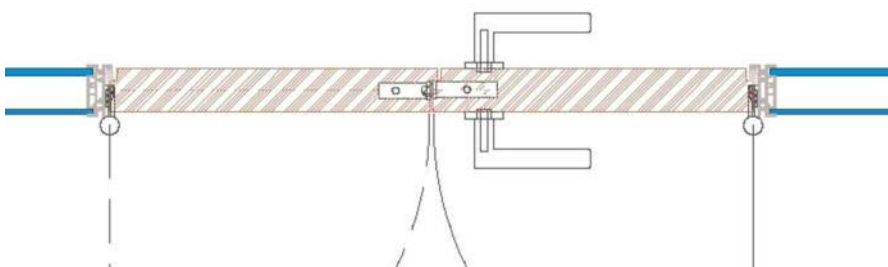
HT2 1000 Holztüre 2-flügelig D = 54 mm Rw = 34 dB
